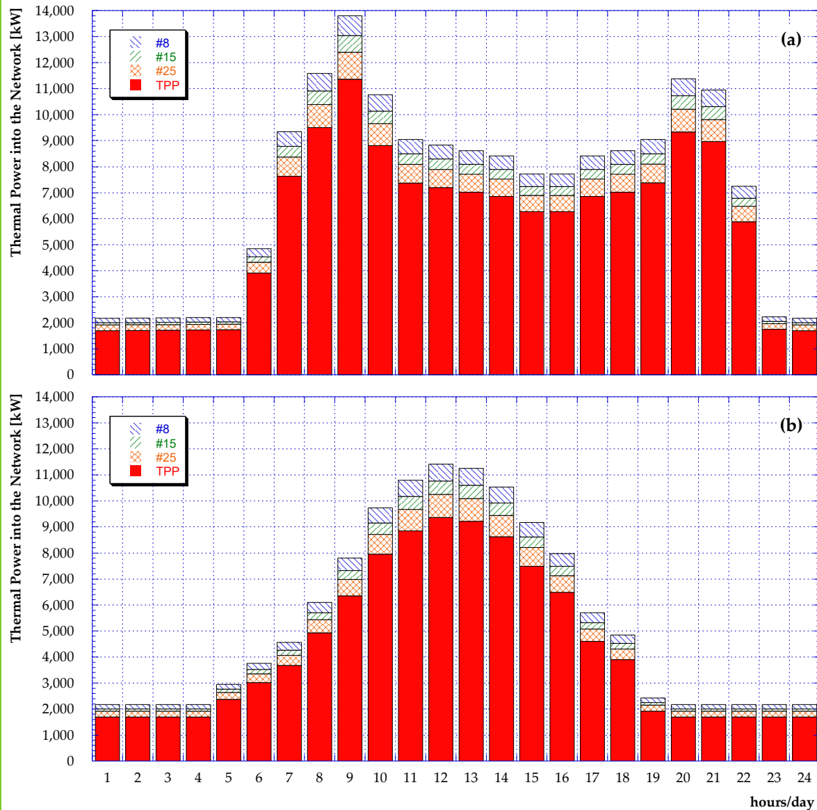
Introduced thermal power into the network by TPP and smart users for (a) typical winter day and (b) middle season and/or summer day
