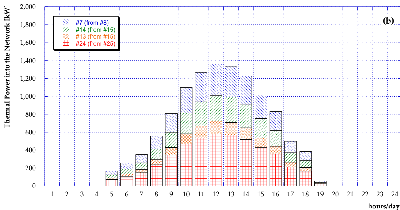
Shared thermal power: served users and sharing smart users for (a) typical winter day and (b) middle season and/or summer day
